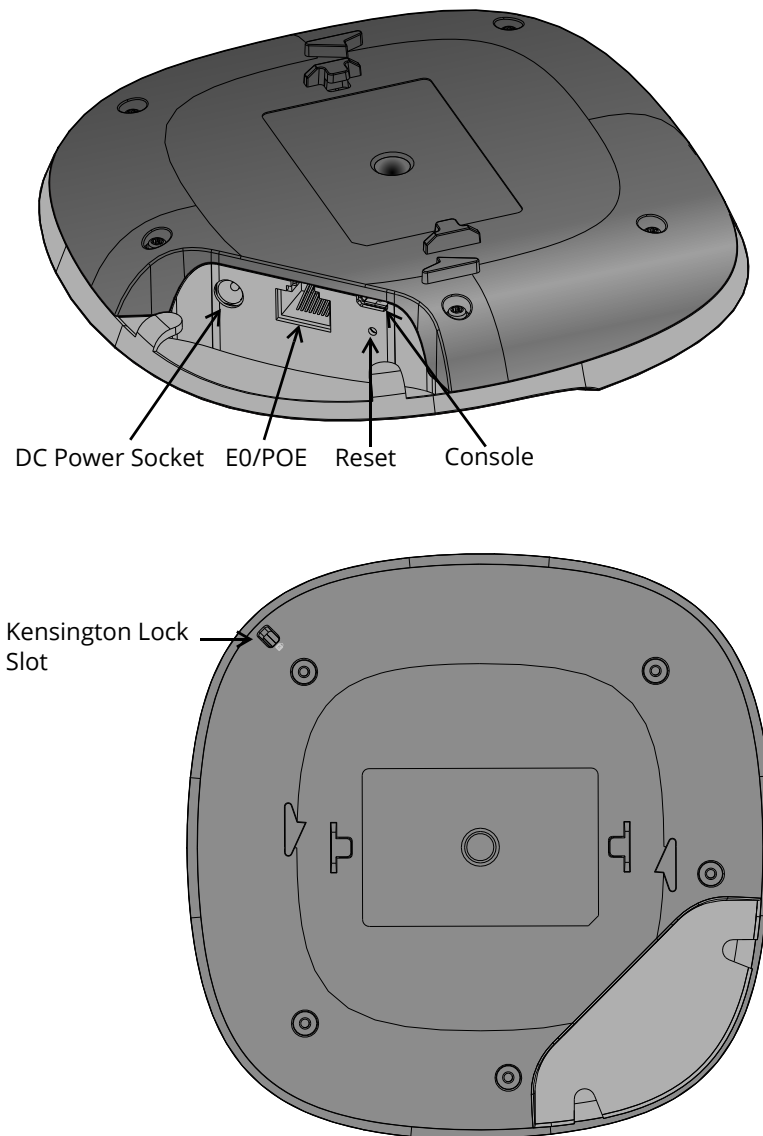
Figure 2 303 Series (rear view)
