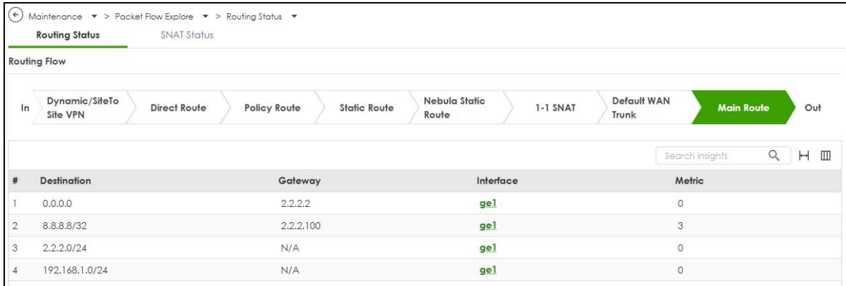
Figure 359 Maintenance > Packet Flow Explore > Routing Status (Main Route)
