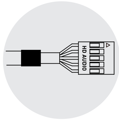
HD Audio Header
