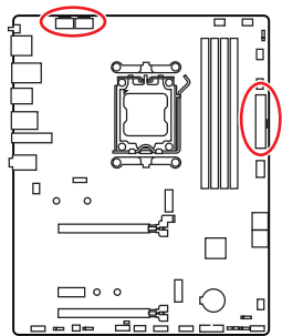
CPU_PWR1, CPU_PWR2
