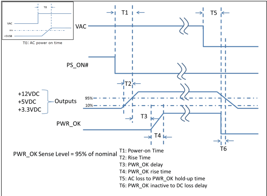
Figure 1 Time Diagram
