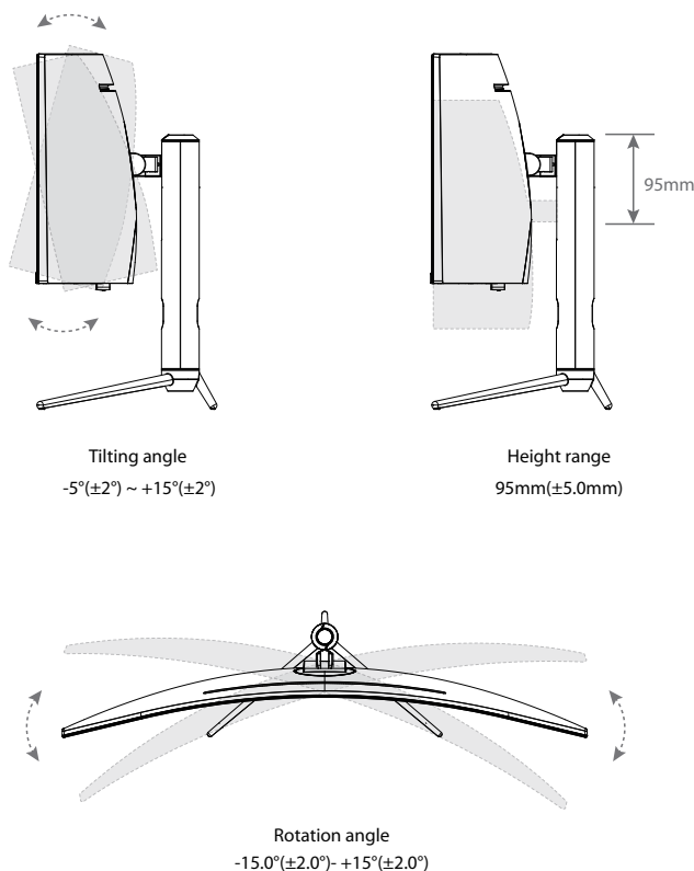
Figure 2-1 Angle Adjustment
