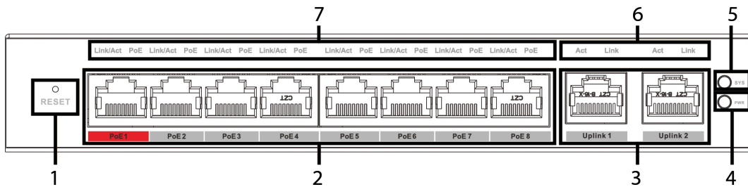
Figure 2-2 Front panel (16-port)
