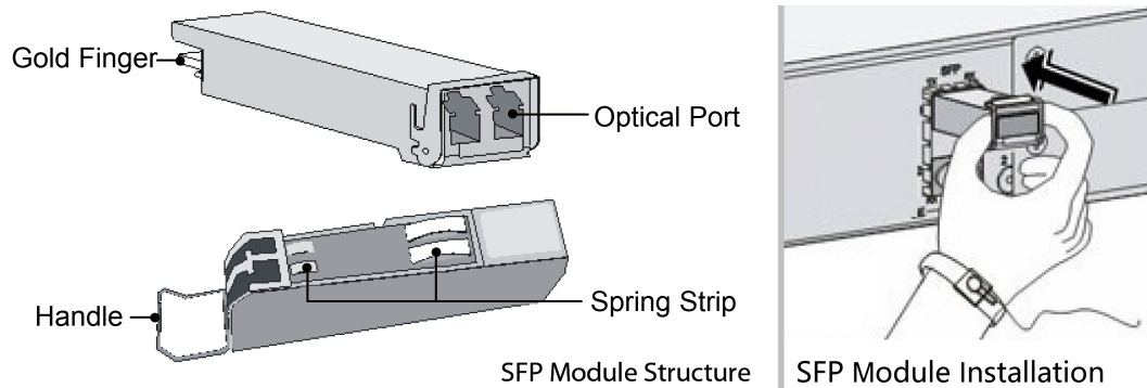
Figure 4-4 SFP module structure and installation
