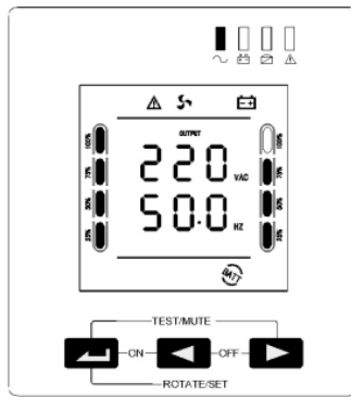
Figure 8. Screen with UPS control buttons
