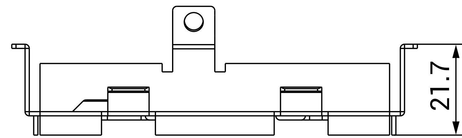
6 BOTTOM VIEW
