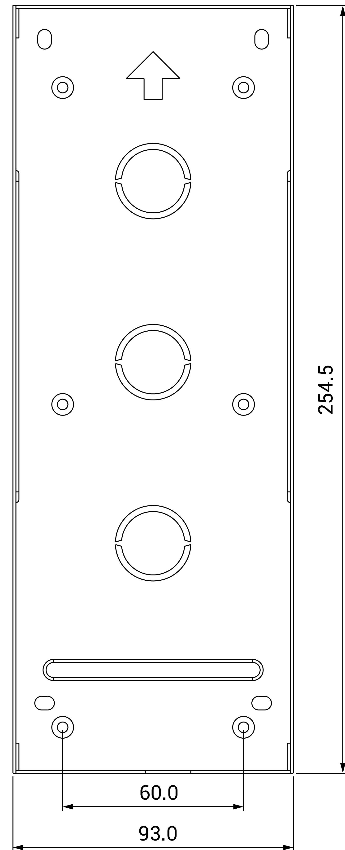
1 FRONT VIEW
