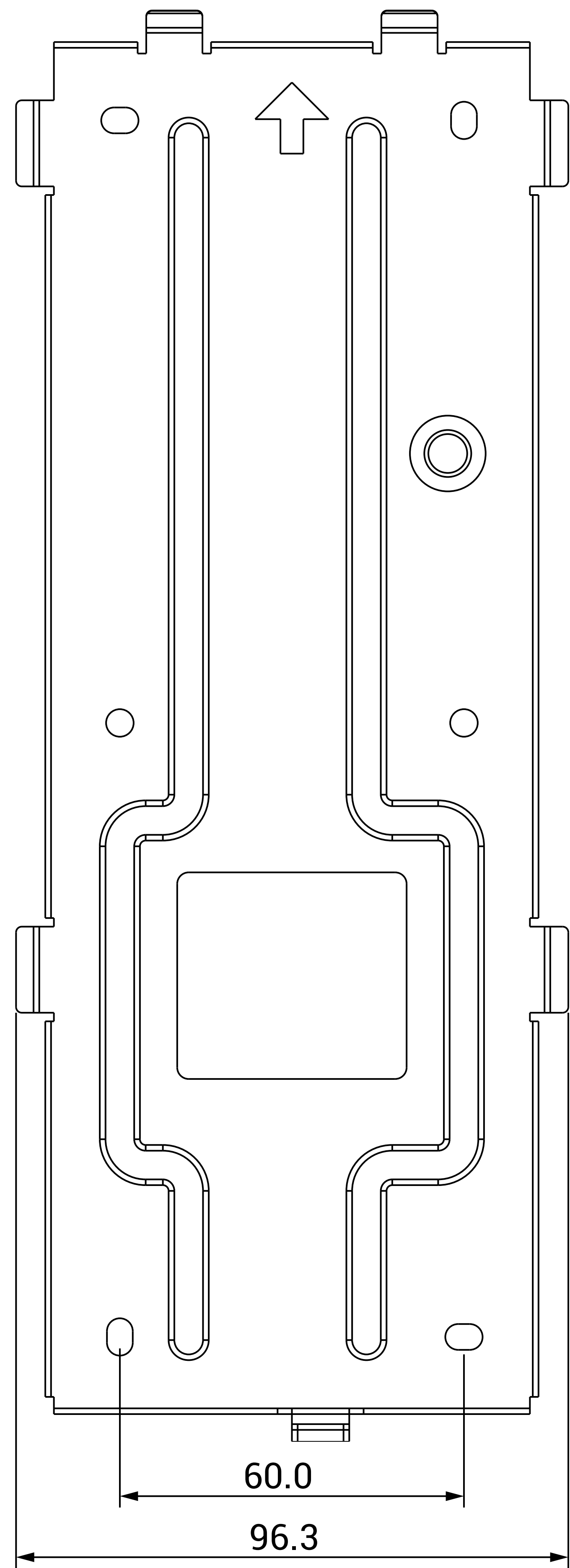
1 FRONT VIEW
