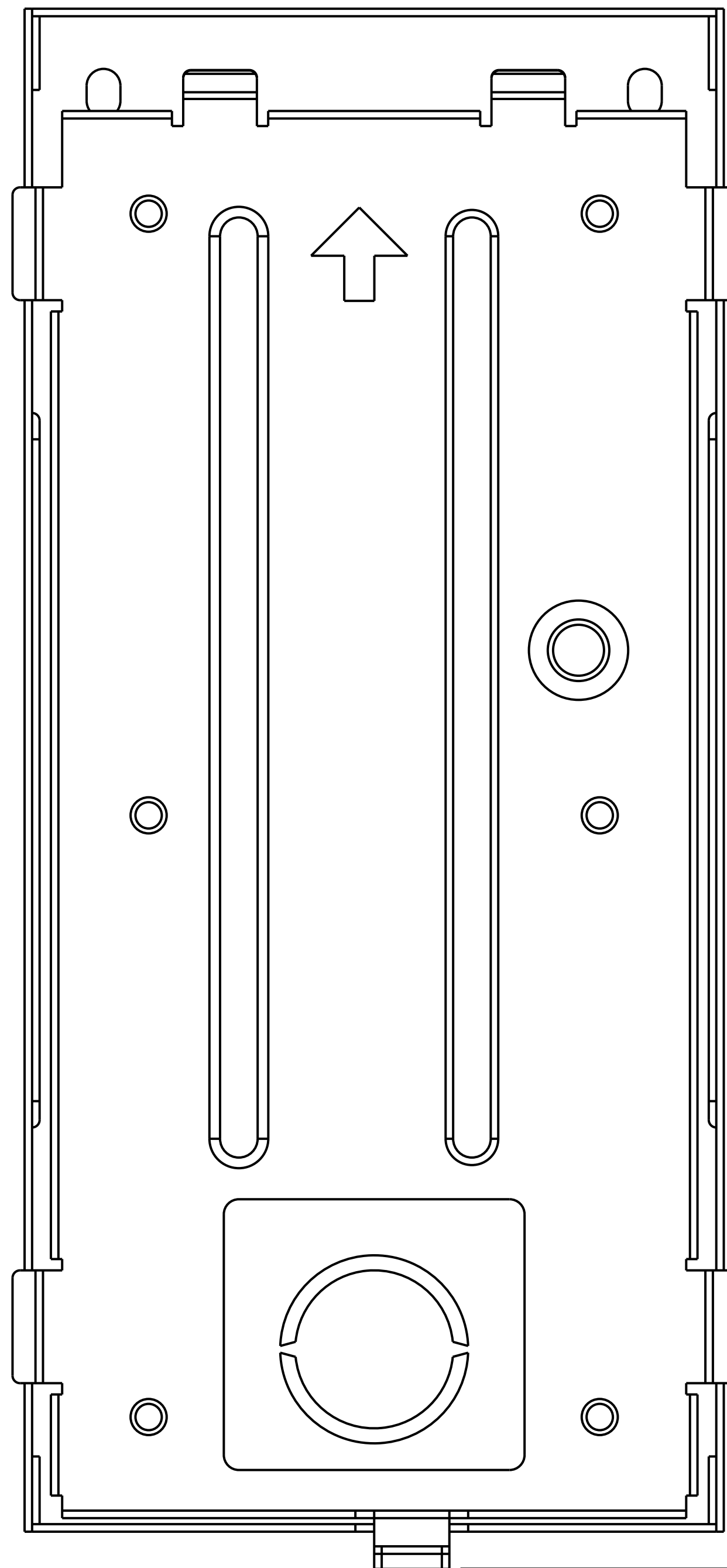
2 FRONT VIEW:FLUSHING MOUNTING BOX PLACEMENT
