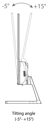
Figure 2-1 Angle Adjustment
