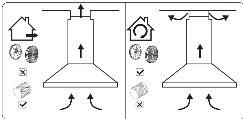
Kanalinstallation
